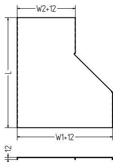
右偏異徑接頭蓋板 Right Reducer Cover
