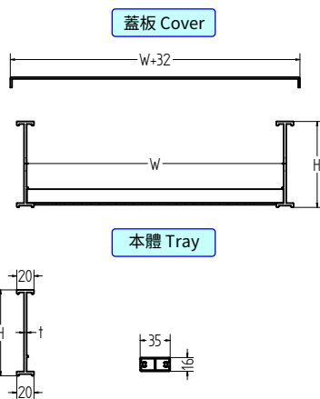
邊槽 Rail
