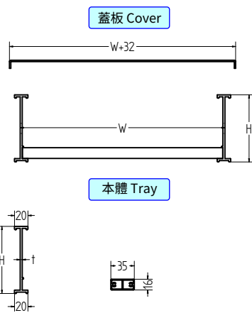
邊槽 Rail
