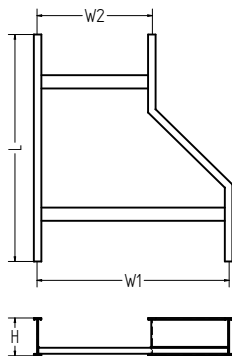
右偏異徑接頭 Right Reducer
